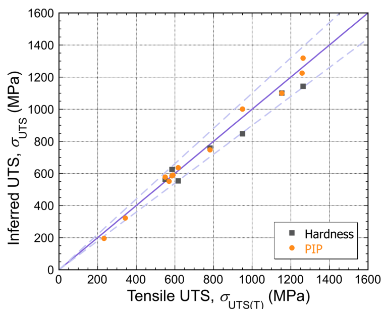
Figure 1: Plot of inferred UTS from PIP and hardness testing using BS ISO-18265:2013 against corresponding tensile tests.
