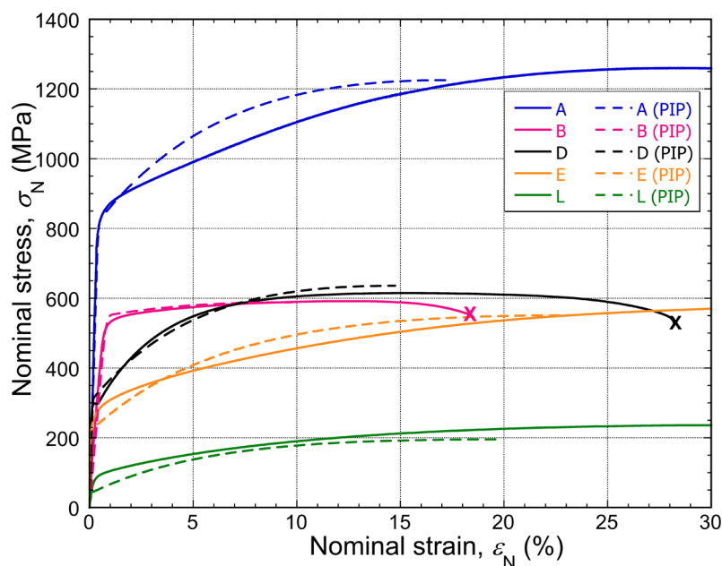
Figure 2: Nominal stress – nominal strain curves for selected materials, from tensile testing and from PIP. The latter are shown only up to the onset of necking (peak in the plot).
